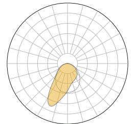
DA5025: Asymmetric 50° at 25° Tilt
